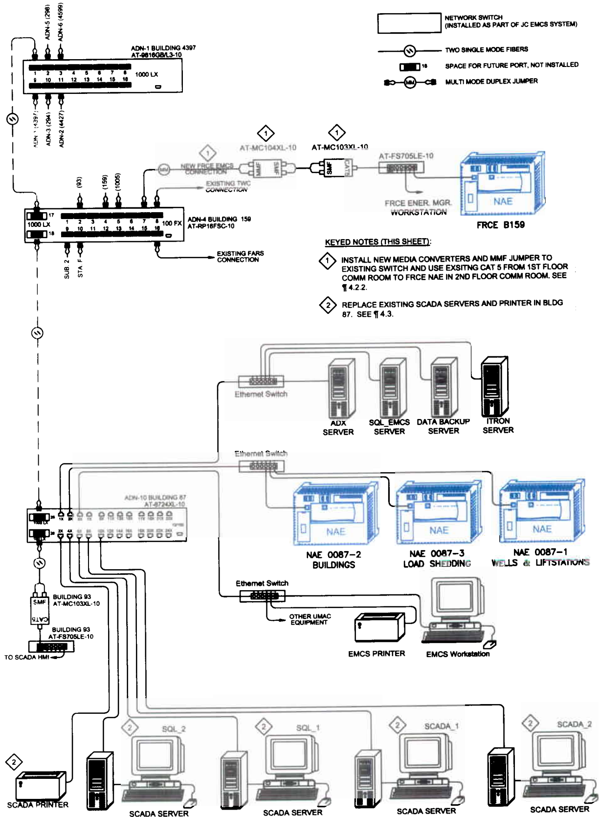
FIGURE 2 - SCADA SERVER REPLACEMENT & BRIDGE TO FRCE
