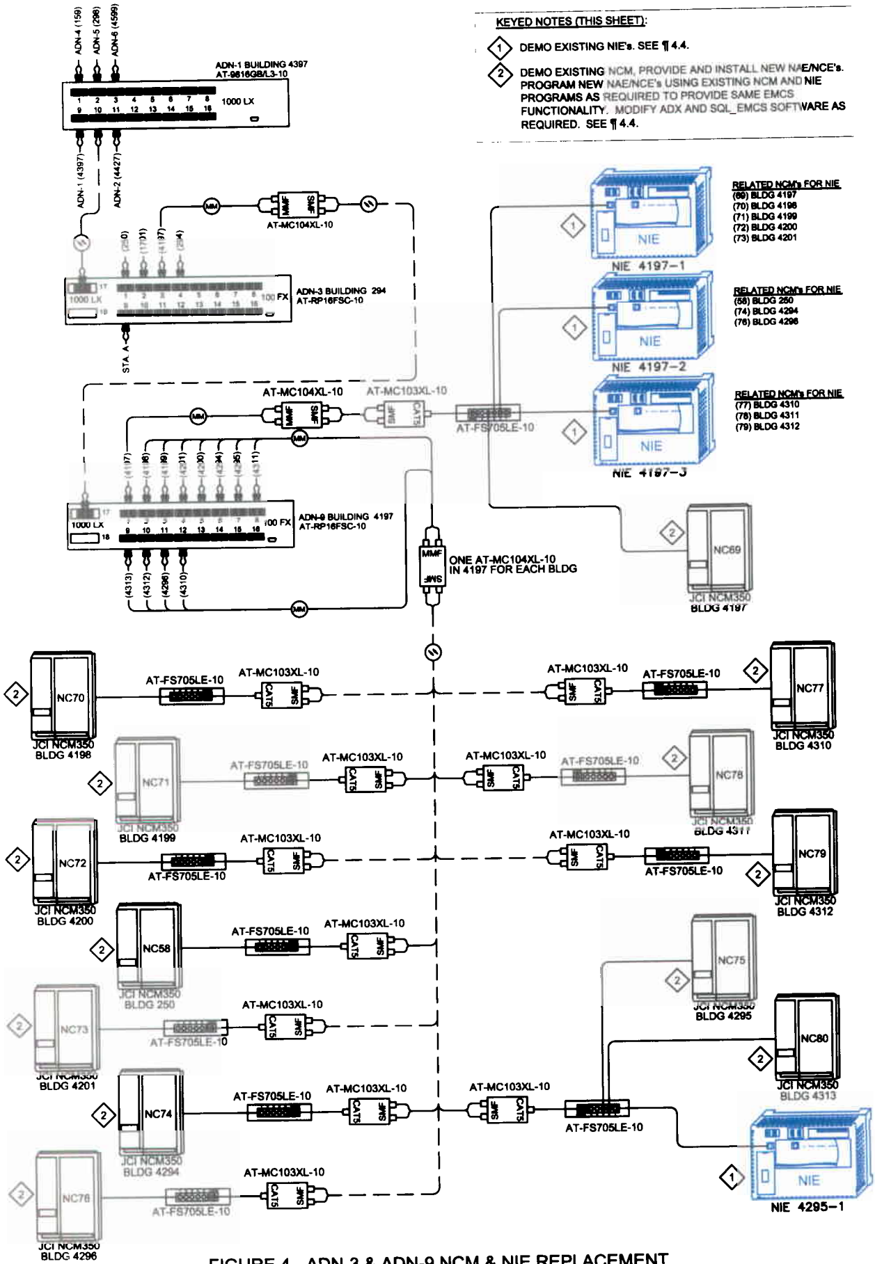
FIGURE 4 - ADN-3 & ADN-9 NCM & NIE REPLACEMENT
