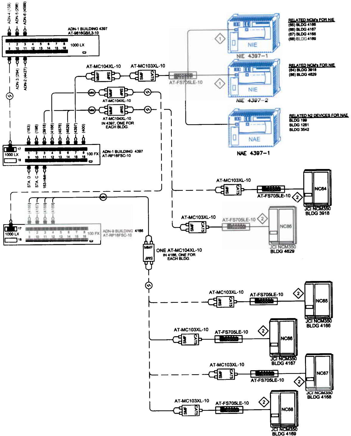
FIGURE 3 - ADN-1 & ADN-9 NCM AND NIE REPLACEMENT
